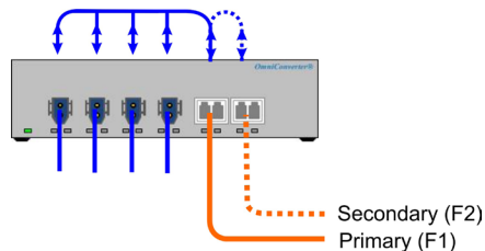
Redundant Uplink
